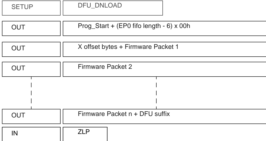
Figure 6. Example of Firmware Download Zero Length DFU_DNLOAD Request
