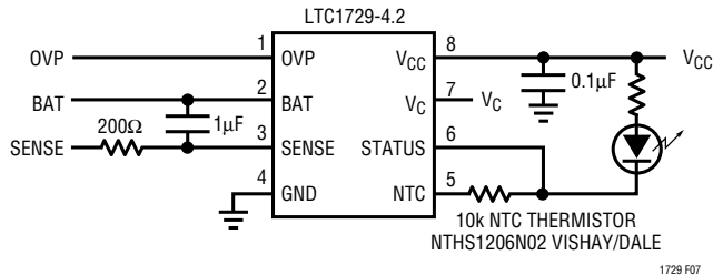
Figure 7. Terminate Charging at C/10
