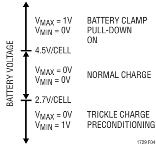
Figure 4. BAT Voltage Operating Range
