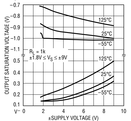
V + ± Output Swing vs Supply Voltage
