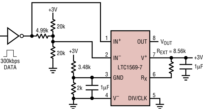
Pulse Shaping Circuit for Single 3V Operation, 300kbps 2 level data, 150kHz Cutoff Filter
