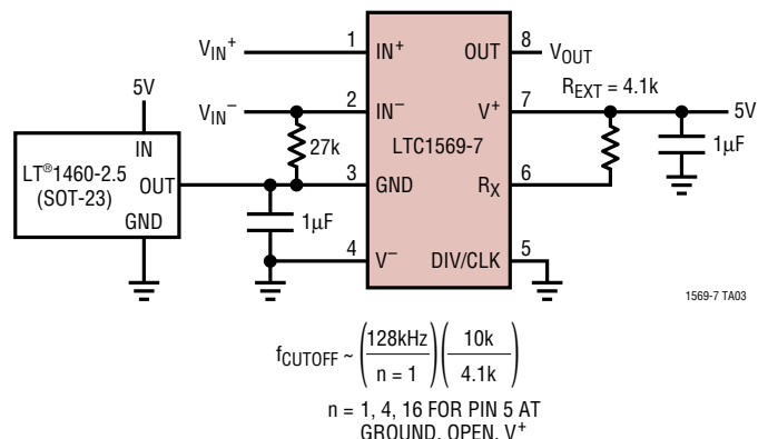
Single 5V Operation, 300kHz Cutoff Frequency, DC Coupled Differential Inputs with Balanced Input Impedance
