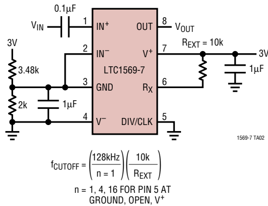
Single 3V Operation, AC Coupled Input, 128kHz Cutoff Frequency
