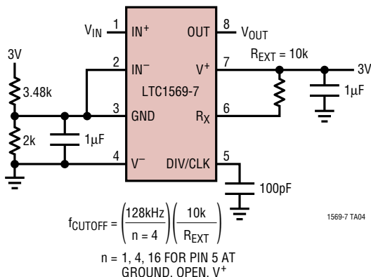
Single 3V Supply Operation, DC Coupled, 32kHz Cutoff Frequency
