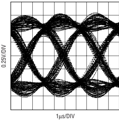
2-Level, 300kbps Eye Diagram
