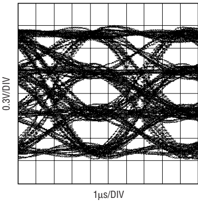
4-Level, 400kbps (200ksps) Eye Diagram
