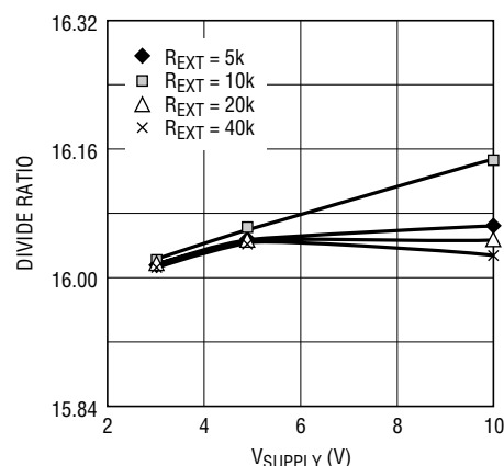
Figure 6. Typical Divide Ratio in the Divide-by-16 Mode, T_A = 25^\circ C
