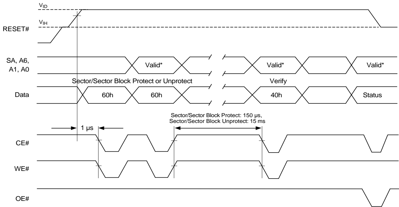
Figure 25. Sector/Block Protect/Unprotect Timing Diagram
