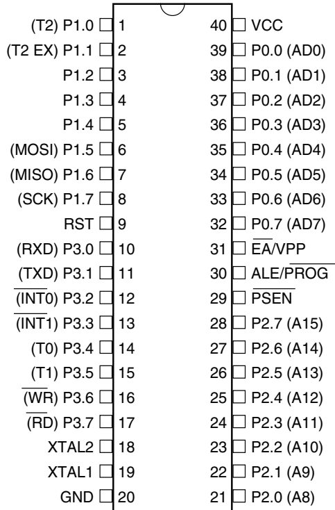
PDIP
