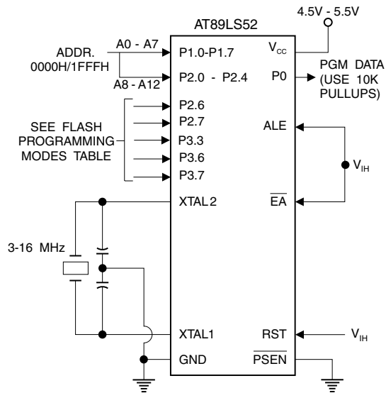
Figure 10. Verifying the Flash Memory (Parallel Mode)
