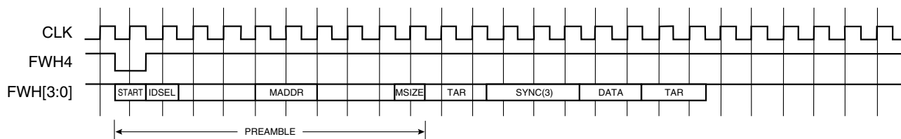
Figure 2. FWH Single-byte Read Waveforms
