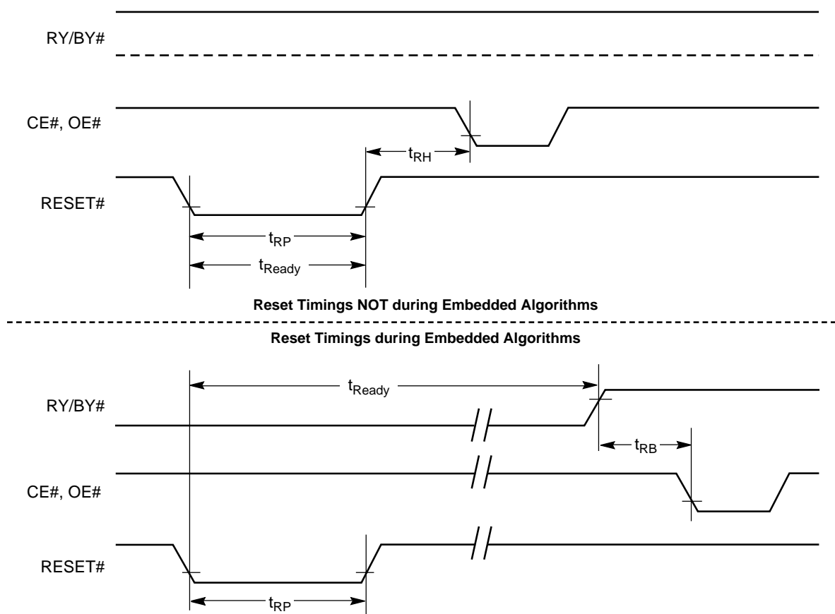
Figure 13. Reset Timings
