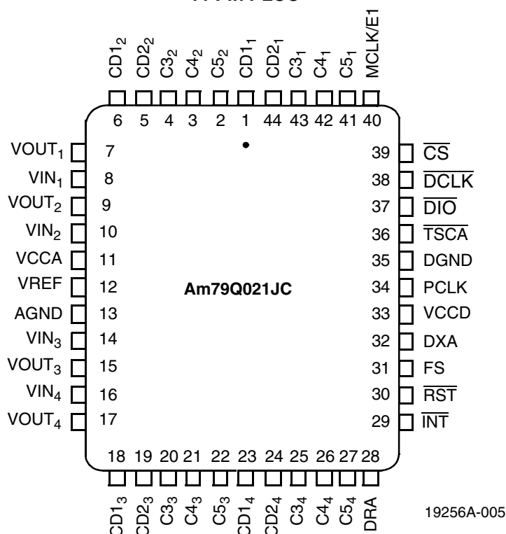
44-Pin PLCC
