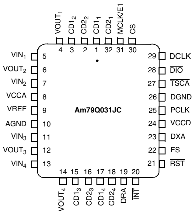
32-Pin PLCC
