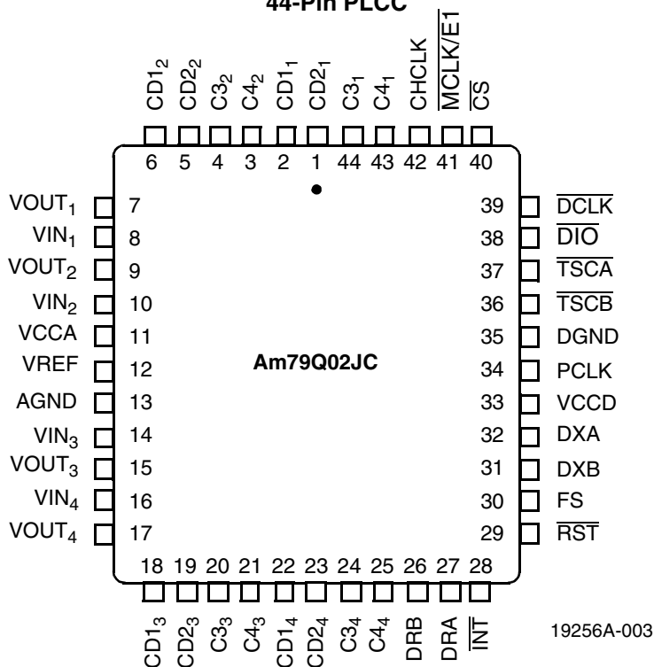
44-Pin PLCC
