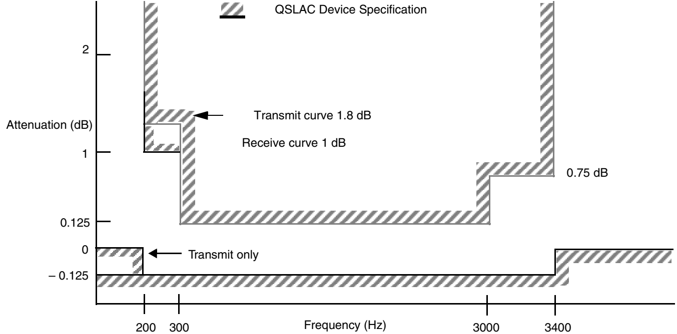
Figure 1. Attenuation Distortion
