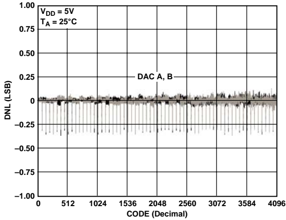
Figure 7. Differential Nonlinearity Errors
