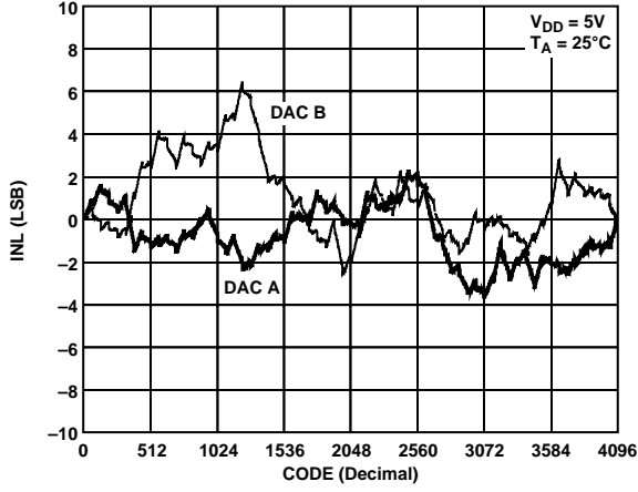
Figure 6. Integral Nonlinearity Errors
