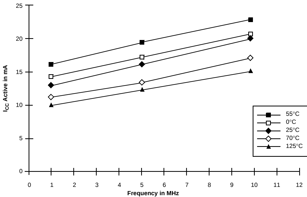
Figure 7. Am28F512A—Average I_{CC} Active vs. Frequency
