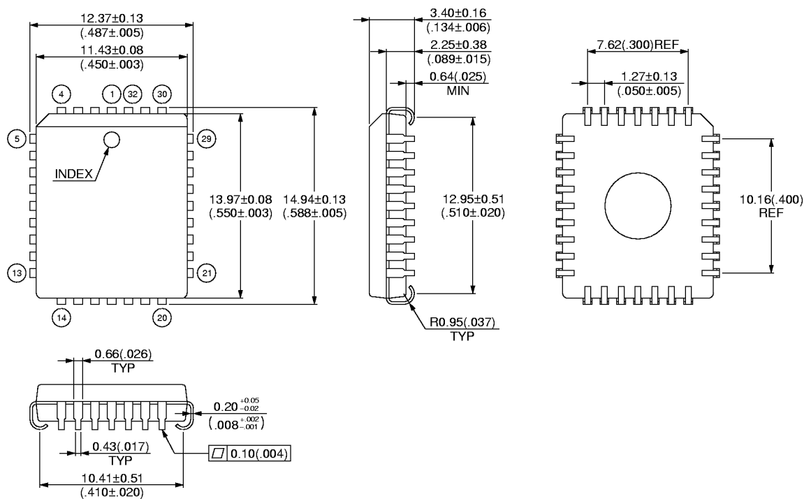
32-Pin Plastic LCC (LCC-32P-M02)
