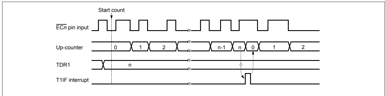
Figure 12-5 Event Counter Mode Timing Chart
