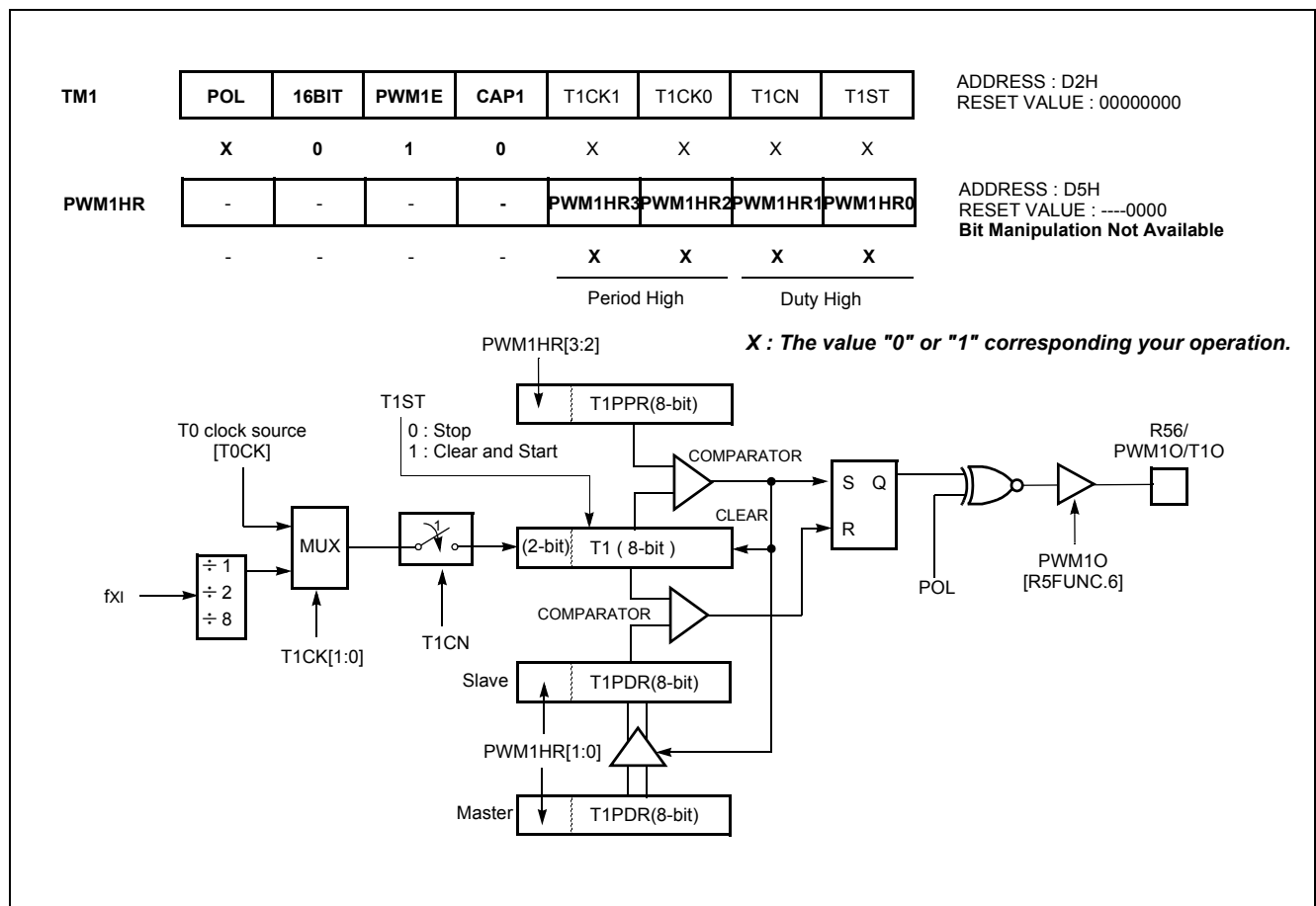
Figure 12-12 PWM Mode
