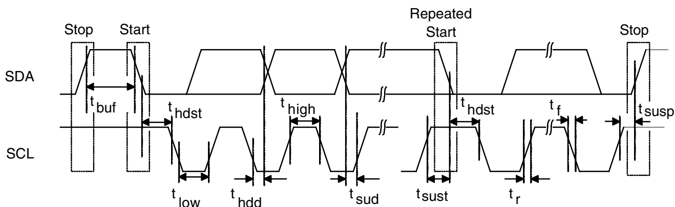
Figure 4. Two-Wire Mode timing
