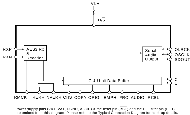
Figure 9. Hardware Mode
