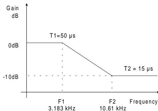
Figure 5. De-Emphasis Curve
