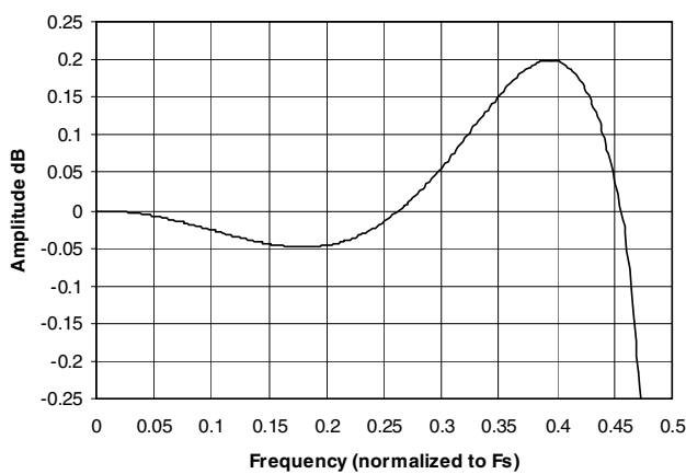
Figure 22. Double-Speed Frequency Response
