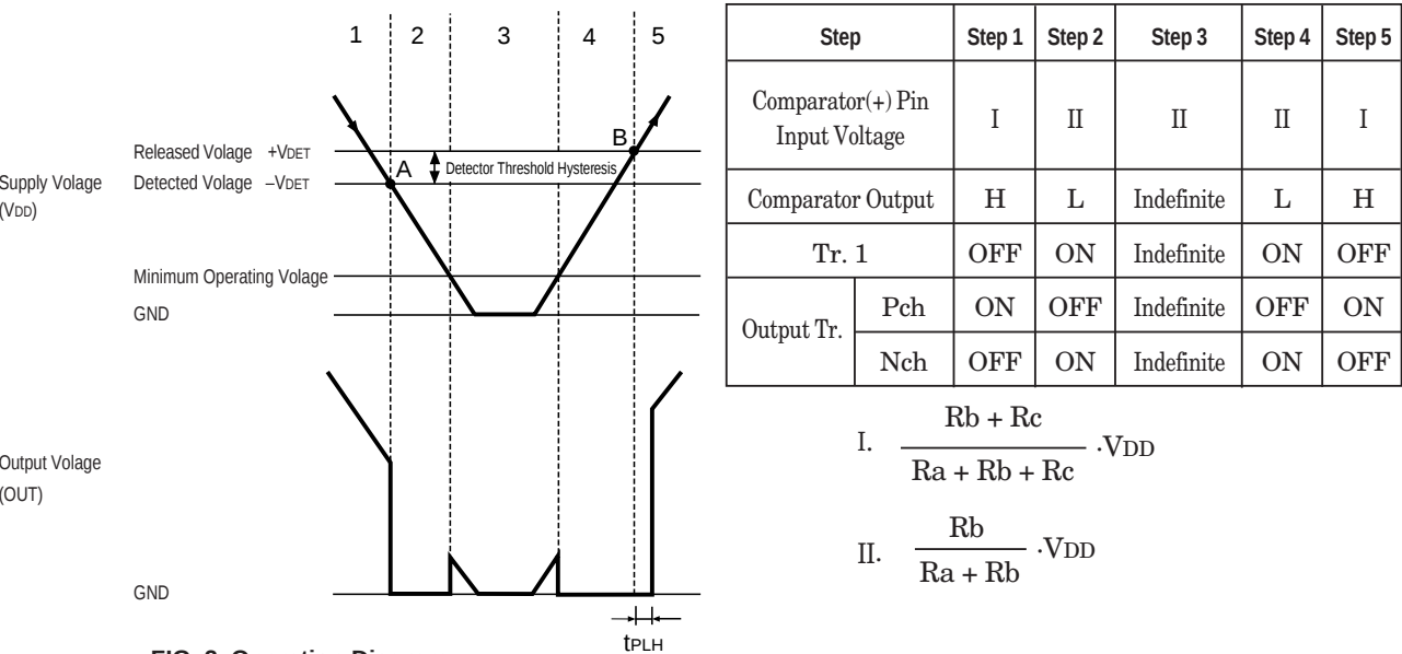
FIG. 2 Operation Diagram
