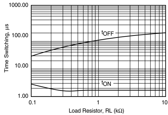
Fig. 9 Switching Time vs. Load Resistor
