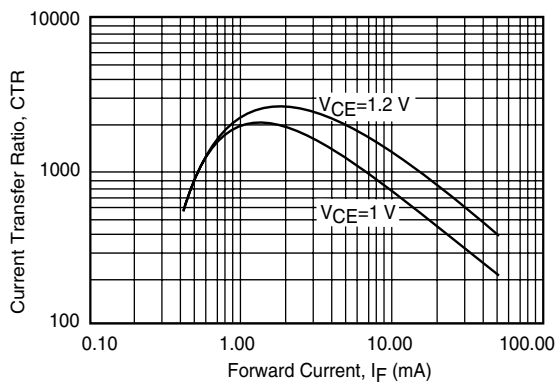
Fig. 7 Current Transfer Ratio vs. Forward Current
