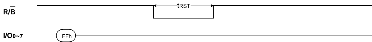
Figure 11. RESET Operation
