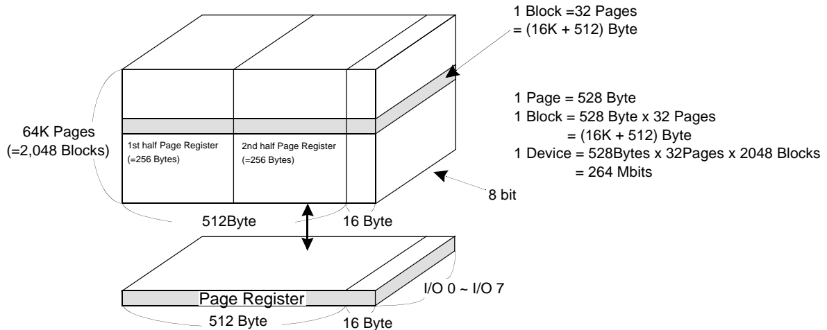
Figure 2. ARRAY ORGANIZATION
