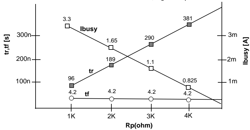
Fig 12 Rp vs tr ,tf & Rp vs i busy
