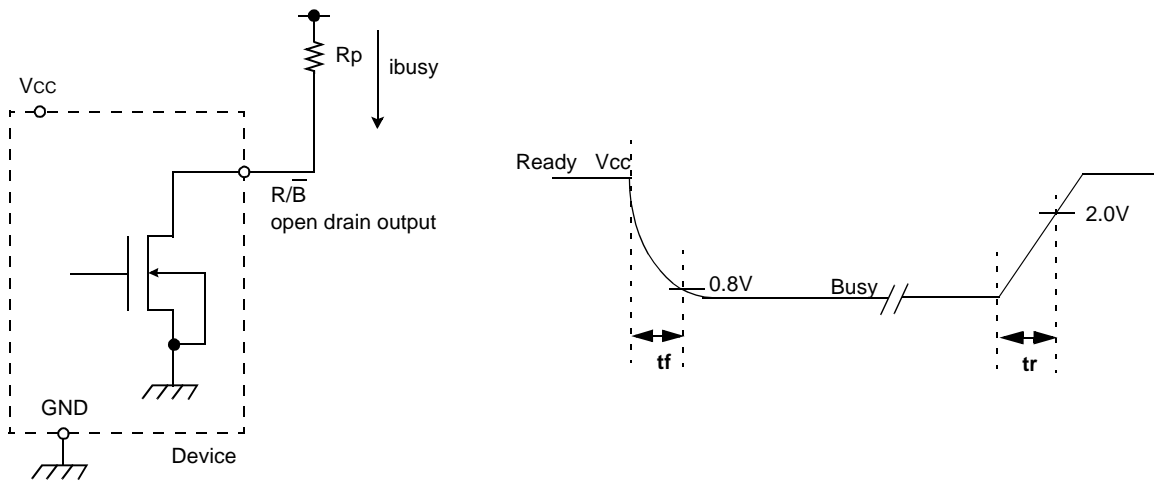
Fig 12 Rp vs tr ,tf & Rp vs i busy
