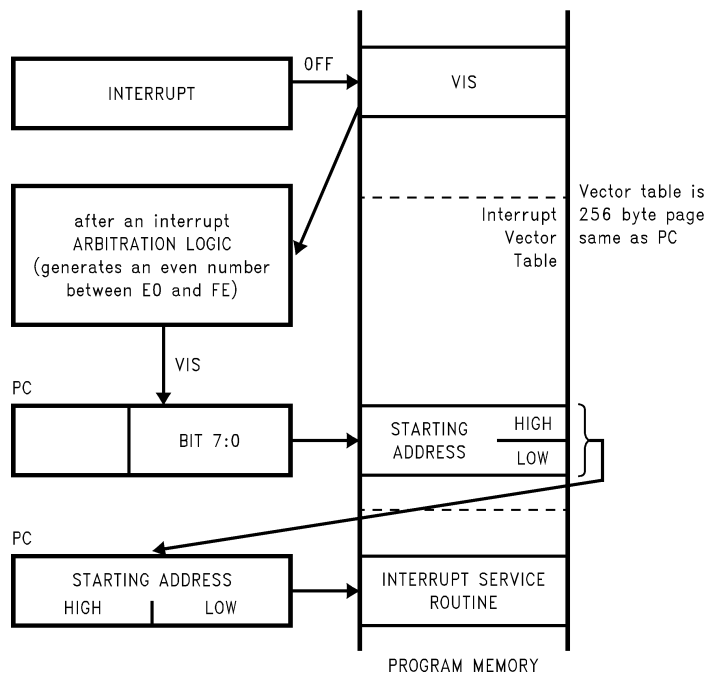
FIGURE 26. VIS Operation
