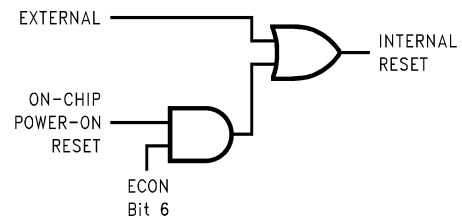
FIGURE 8. Reset Logic
