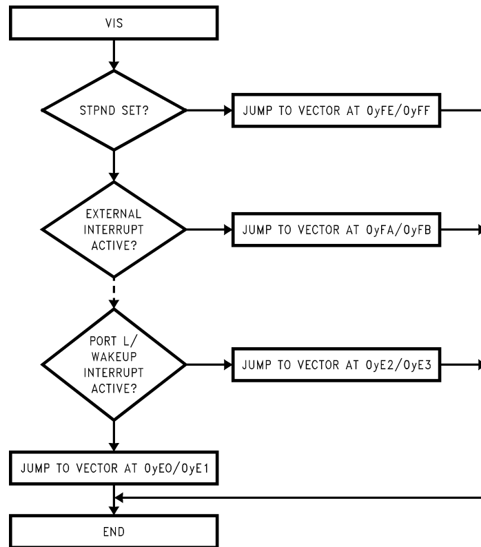
FIGURE 27. VIS Flowchart
