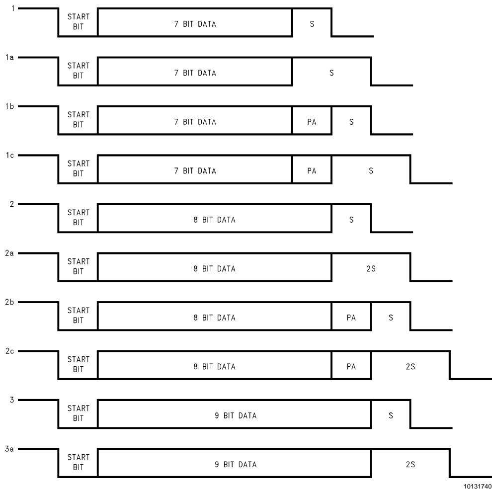
FIGURE 22. Framing Formats
