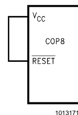
FIGURE 11. Reset Circuit Using Power-On Reset
