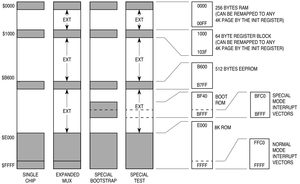
Figure 5 Memory Map
