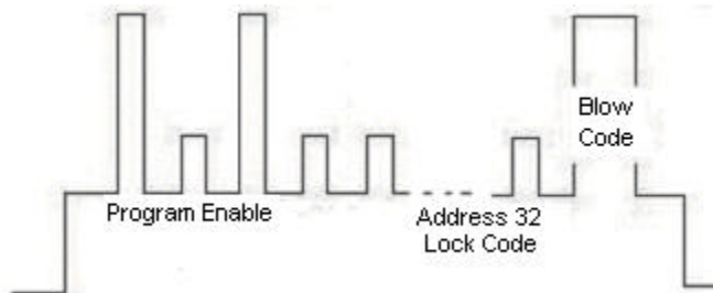
Figure 4. Lock-bit programming
