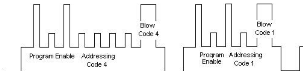
Figure 3. Bit programming.
