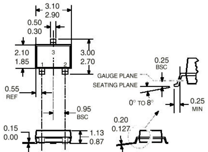
Dimensions in Millimeters (controlling dimensions)
