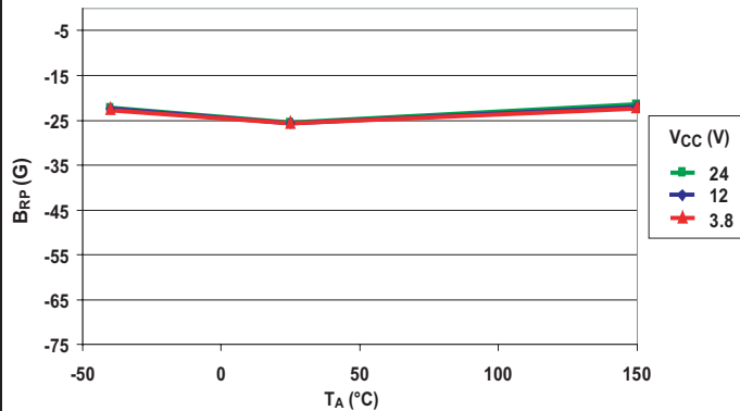
Release Point versus Ambient Temperature (A1202, A1203)
