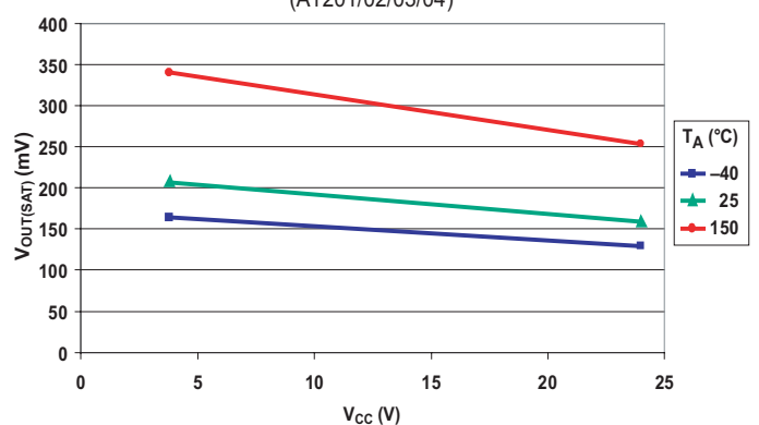
Output Voltage (On) versus Supply Voltage (A1201/02/03/04)
