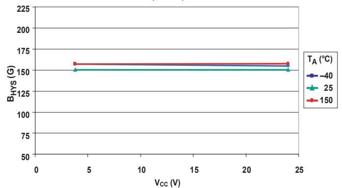
Hysteresis versus Supply Voltage (A1210)
