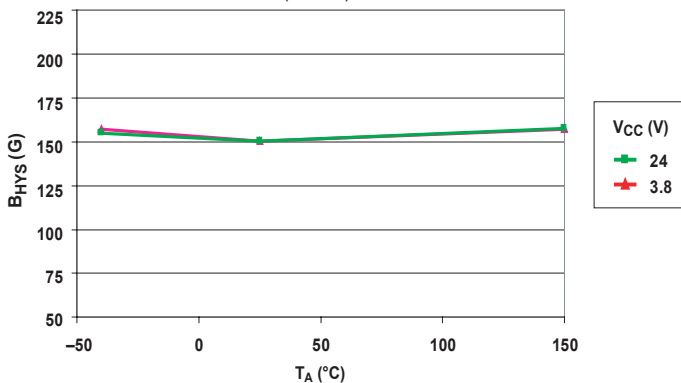
Hysteresis versus Ambient Temperature (A1210)
