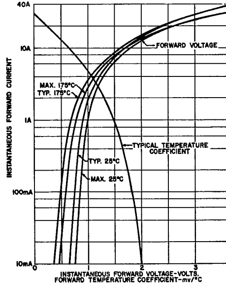
FORWARD CHARACTERISTICS
