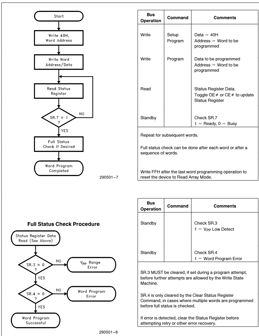
Figure 7. Automated Word Programming Flowchart
