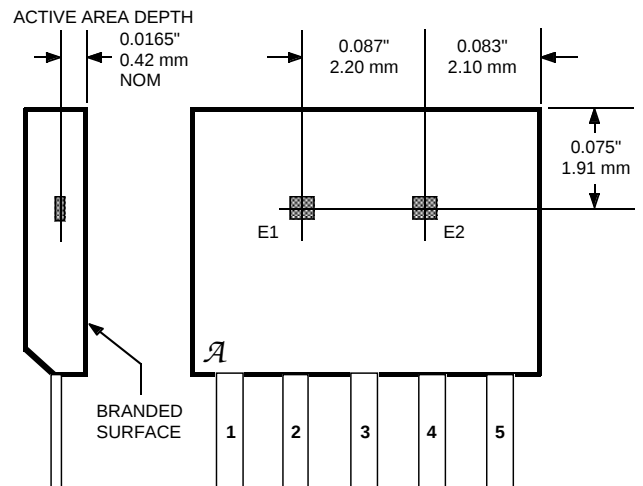
Figure 5 SENSOR LOCATIONS ( \pm 0.005 " [0.13 mm] die placement)
