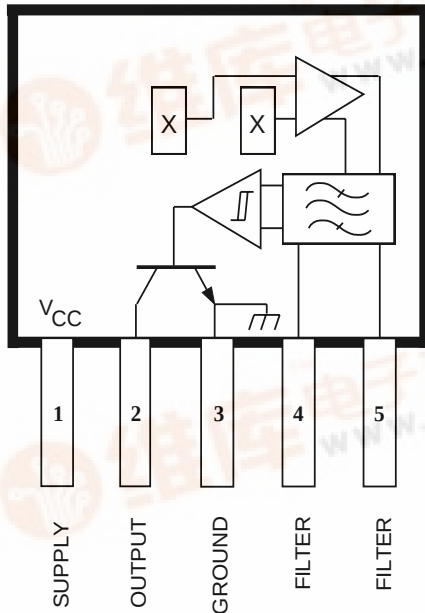
Dwg. PH-011
