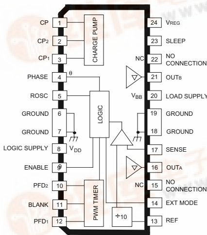
Dwg. PP-069-4
