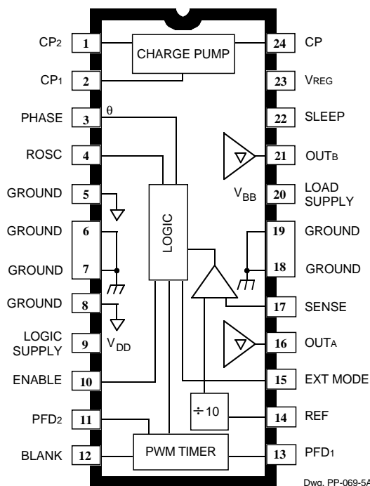
Dwg. PP-069-5A
