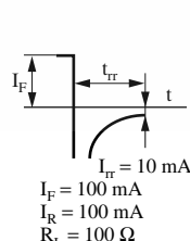
Output Pulse
