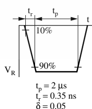
Input Pulse
