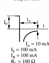
Output Pulse
