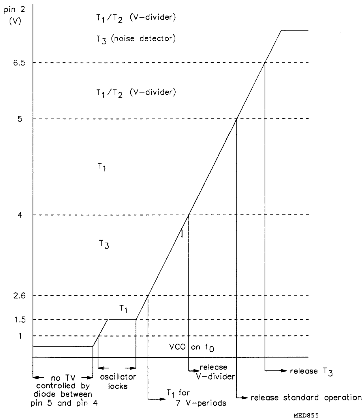
Fig.15 Control of operation states by voltage at pin 2.
