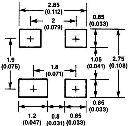
DIMENSIONS: MILLIMETERS (INCHES) SOT-143
