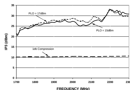
Input IP3 &amp; 1 dB Compression Point
