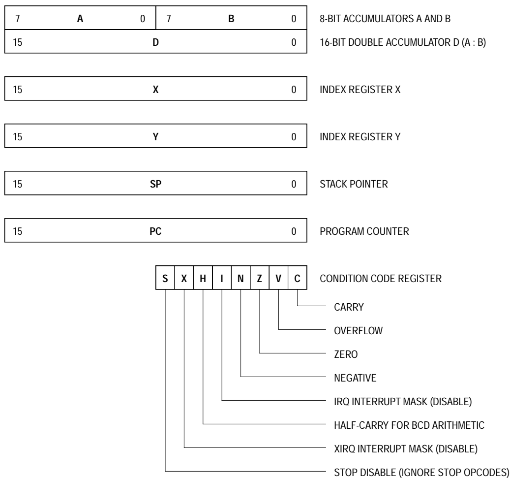
Figure 3-1. Programming Model
