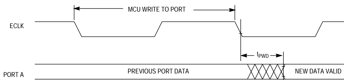
Figure 18-7. Port Write Timing Diagram
