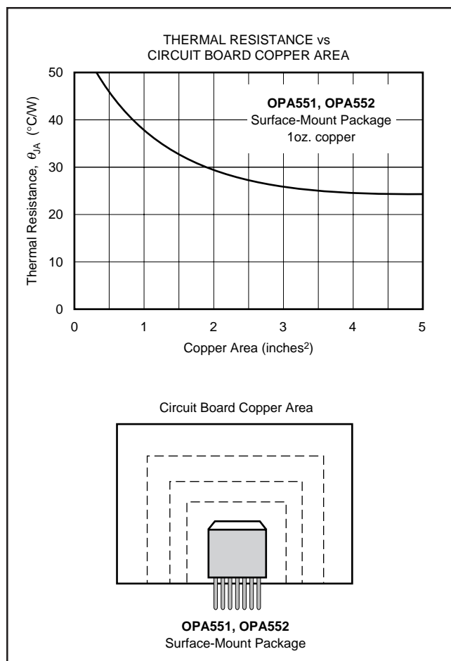
FIGURE 6. DDPAK Thermal Resistance vs Circuit Board Copper Area.
