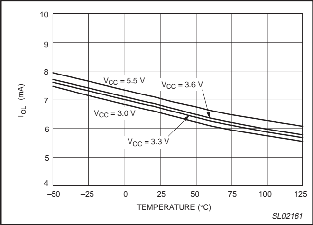
Figure 9. Typical ALERT I_{OL} versus temperature and V_{DD} ( V_{OL} = 0.4\text{ V} )
