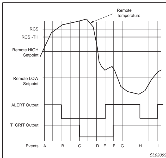
Figure 16. Fault Queue Remote High and Low and \overline{\text{T\_CRIT}} , \overline{\text{T\_CRIT}} Hysteresis setpoint response (Comparator mode)
