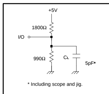
Figure 2. Output Load for t_{CLZ} , t_{CHZ} , t_{OHZ} , t_{WHZ} , and t_{OW}
