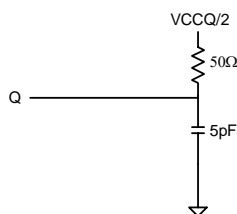
2. Output Load Equivalent
