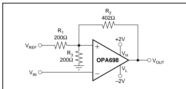
FIGURE 15. Very High-Speed Schmitt Trigger.
