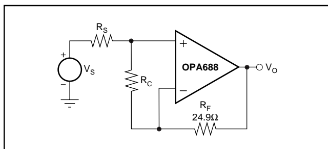
FIGURE 17. Unity-Gain Buffer.
