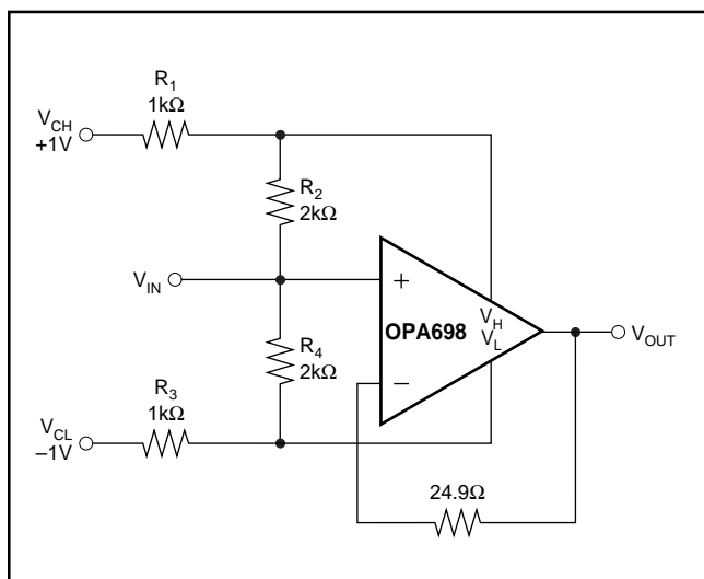
FIGURE 13. Soft-Clipping Circuit.
