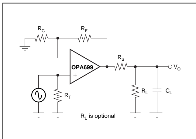
FIGURE 14. Driving Capacitive Loads.
