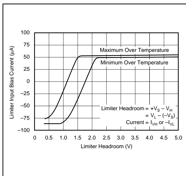
FIGURE 12. Limiter Bias Current vs Bias Voltage.
