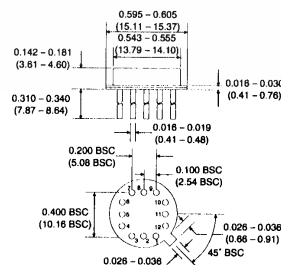
Package Dimensions
