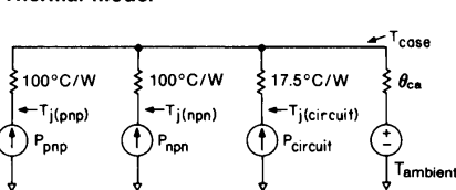
Thermal Model
