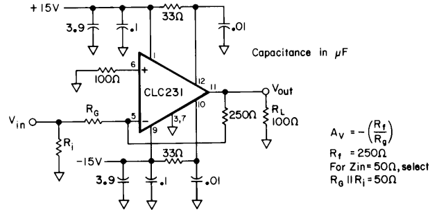
Figure 2: suggested inverting gain circuit
