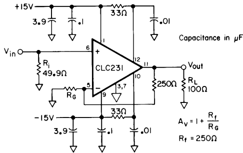
Figure 1: suggested non-inverting gain circuit
