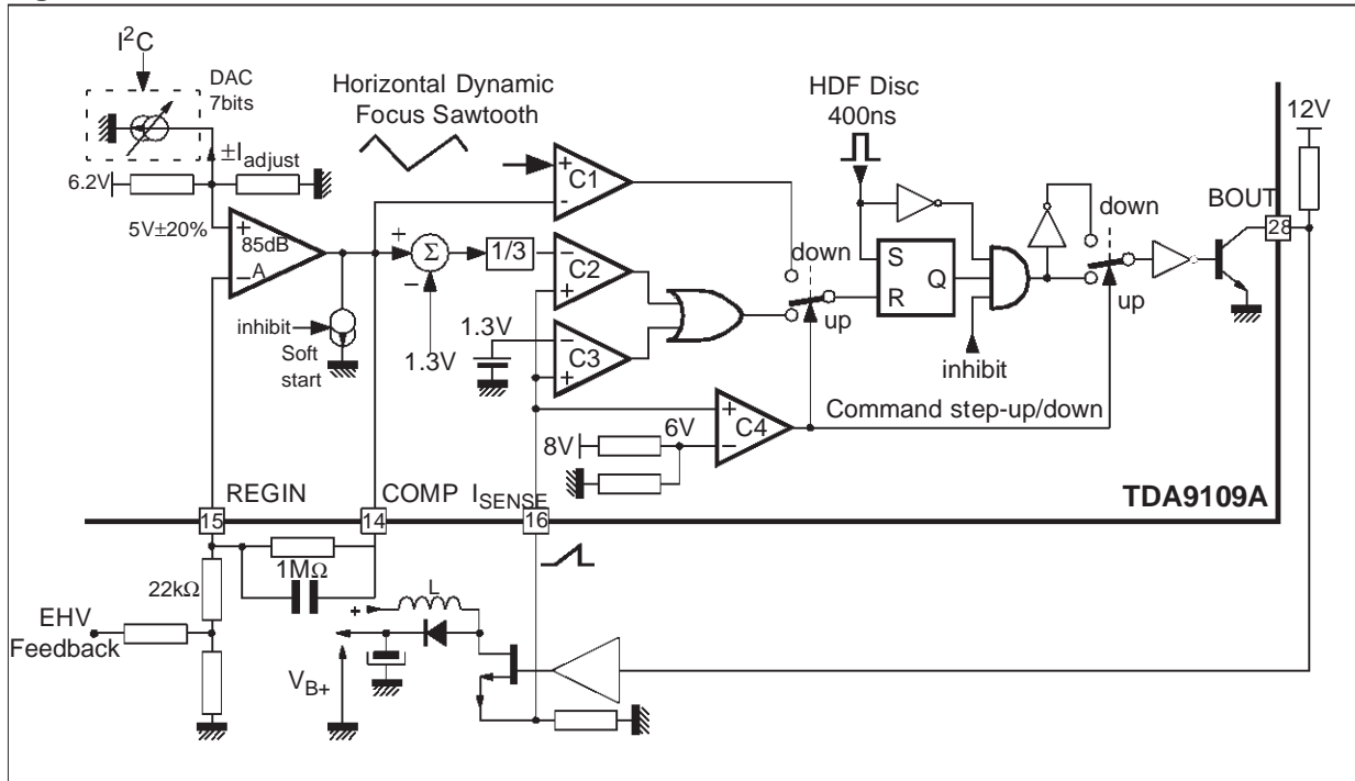
Figure 18. DC/DC Converter
