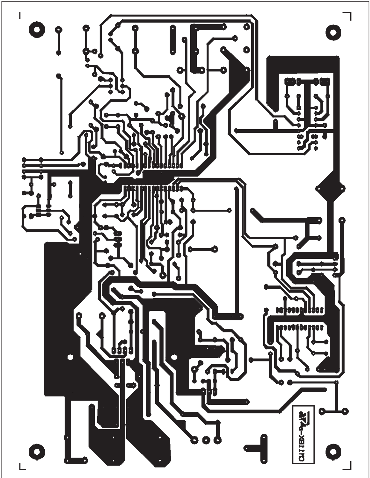
Figure 41. PCB Layout
