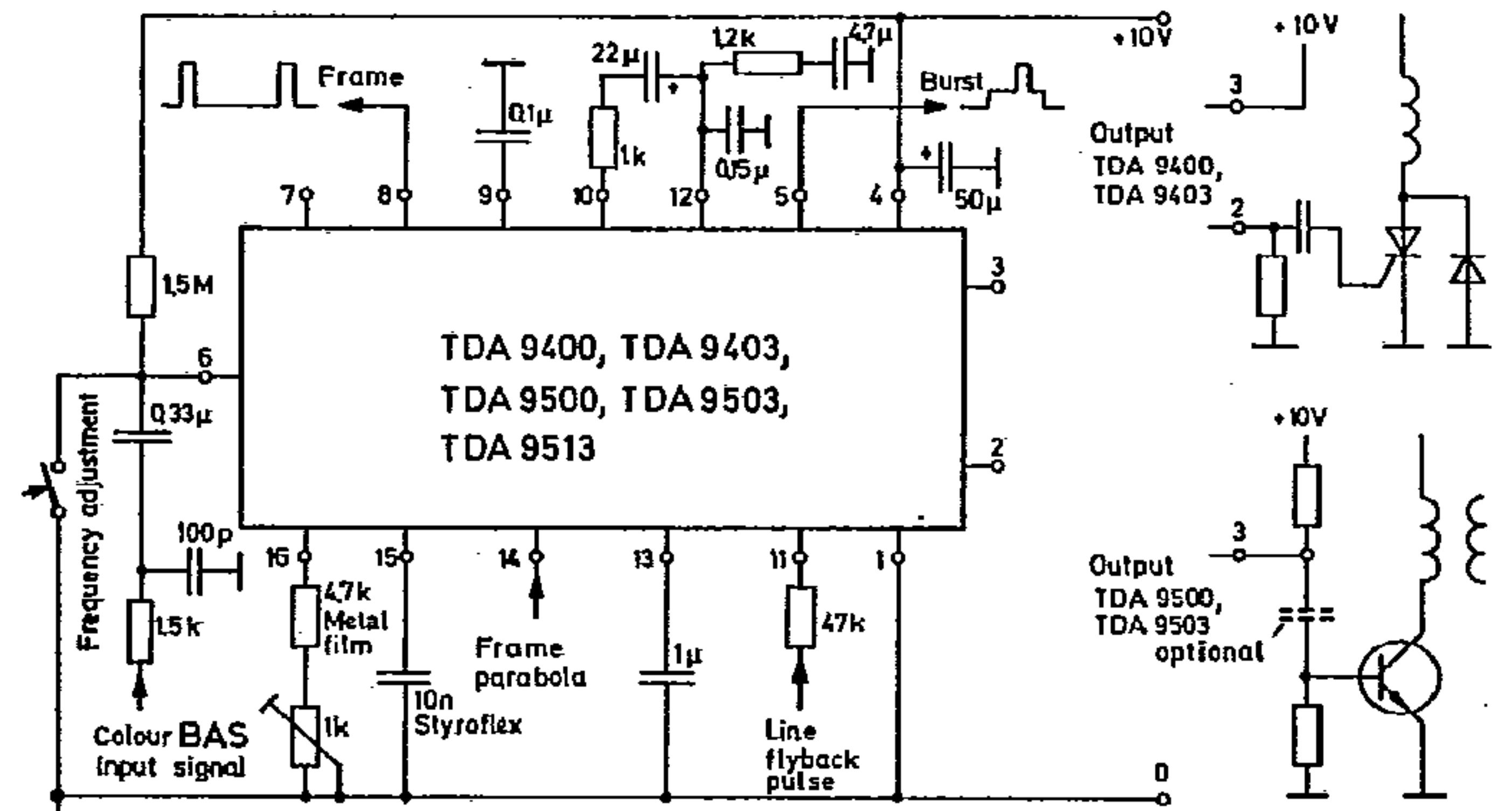
Application Circuit
