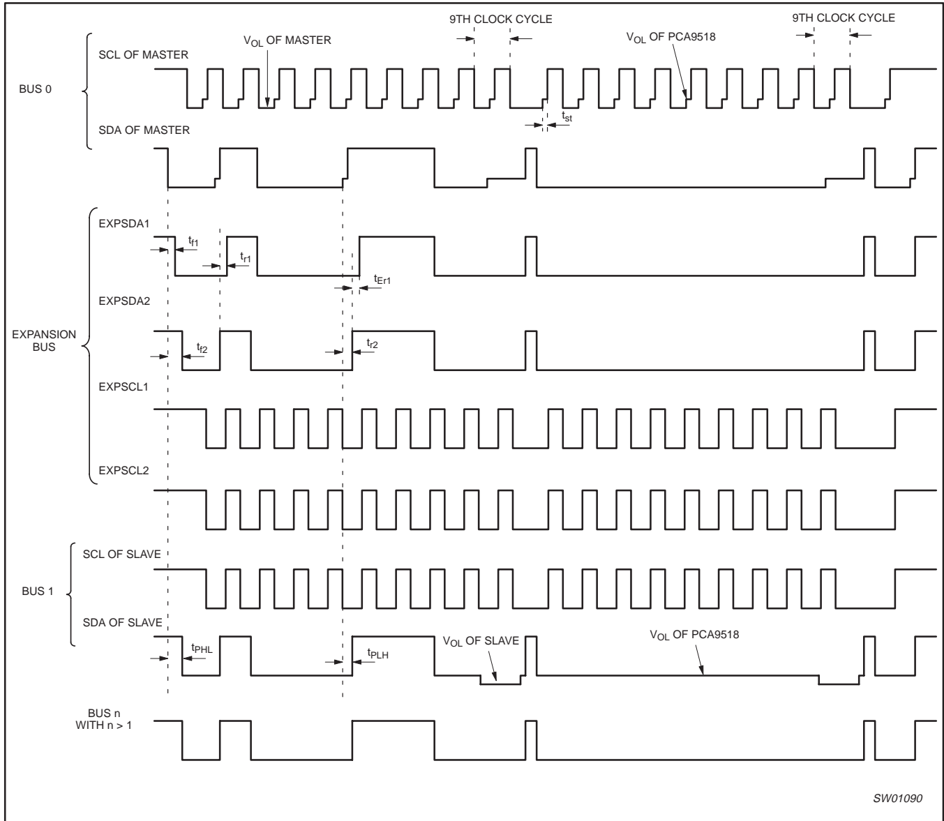
Figure 5. Bus waveforms
