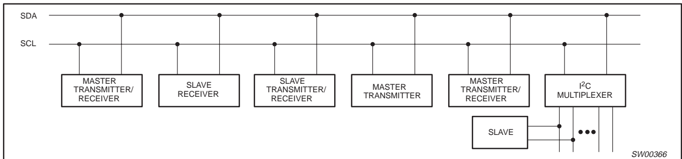
Figure 8. System configuration
