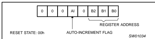
Figure 4. Control register
