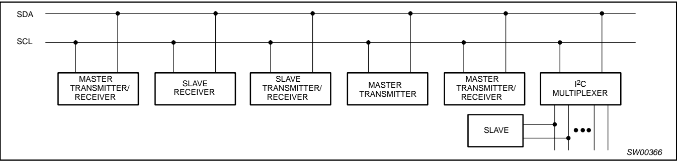
Figure 7. System configuration
