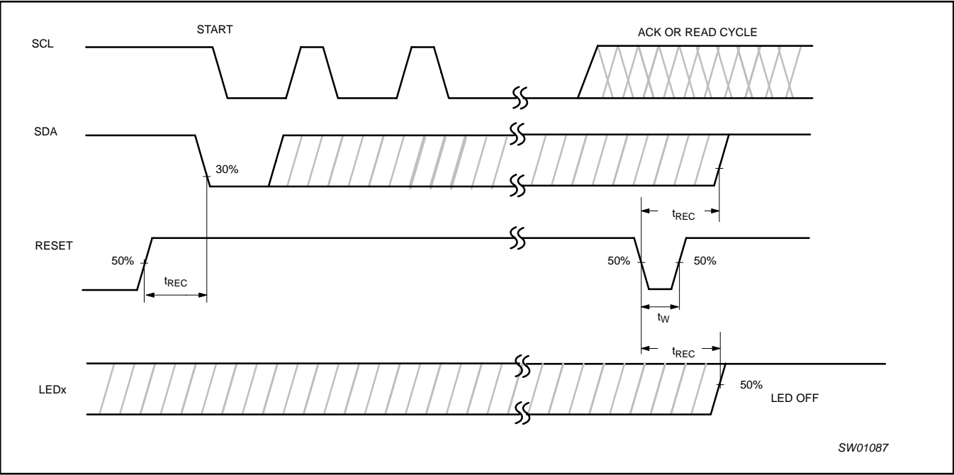
Figure 17. Definition of RESET timing
