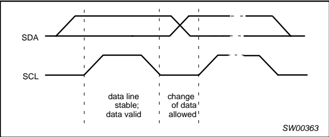
Figure 5. Bit transfer
