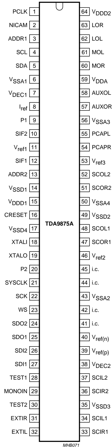
Fig.2 Pin configuration (TDA9875A).
