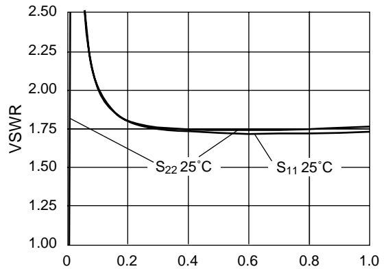
VSWR vs. Frequency 20 dB State
